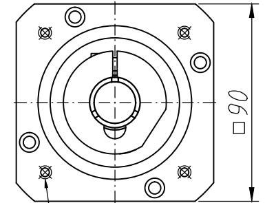
4-M6XP1 PCD \phi 90
