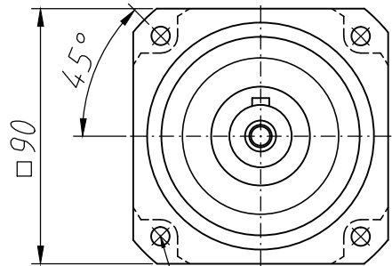
4- \phi 6.5 HOLE PCD \phi 100
